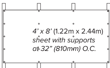
Figure E - Fastener / Fixing Pattern
